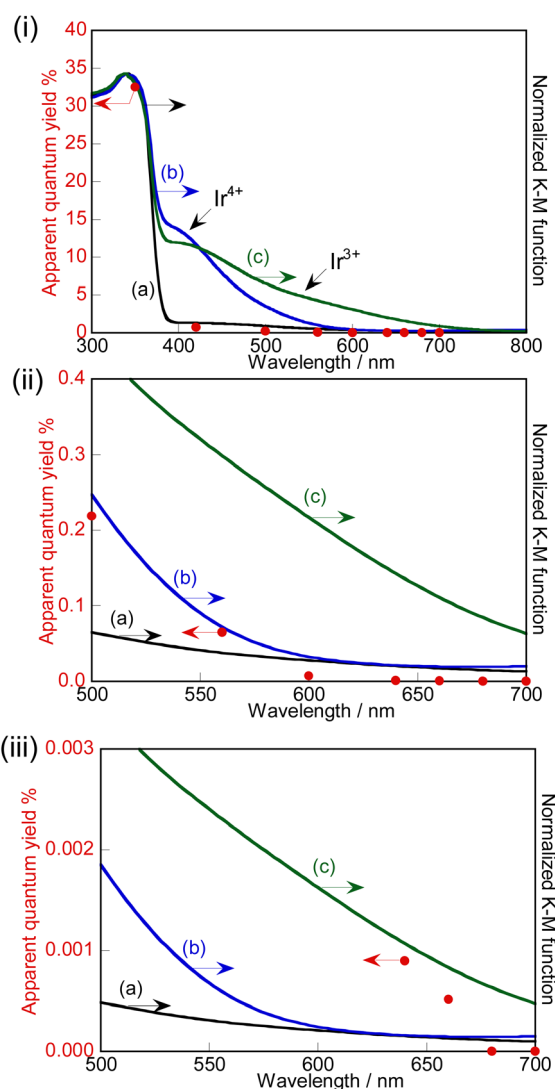
Fig. 4 Action spectrum of photocatalytic water splitting over \text{RhCrO}_x (0.1 mol%)-loaded \text{SrTiO}_3\text{:Ir(0.009\%),Sb(0.018\%),Al} prepared by the flux treatment with \text{Al}_2\text{O}_3 (1%) addition after SSR and diffuse reflectance spectra of (a) \text{SrTiO}_3\text{:Ir(0.009\%),Sb(0.018\%)} prepared by the flux treatment with \text{Al}_2\text{O}_3 (1%) addition after SSR, (b) \text{SrTiO}_3\text{:Ir(0.2\%)} , and (c) \text{H}_2 -reduced (673 K, 1 h) \text{SrTiO}_3\text{:Ir(0.2\%)} . (ii) An enlarged scale of (i); (iii) an enlarged scale of (ii). Photocatalyst: 0.5 g, cocat.: \text{RhCrO}_x (impregnation), reactant solution: pure water (120 mL), light source: a 300 W Xe lamp with band-pass filters, cell: a top-irradiation cell with a Pyrex window, system: a gas-tight circulation system.
