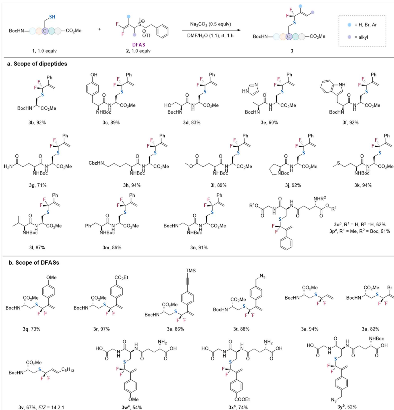
Scheme 1 S-gem -Difluoroallylation of cysteine-containing dipeptides and tripeptides with DFAS 2. a a Reaction conditions: 1 (0.2 mmol, 1.0 equiv.), 2 (1.0 equiv.), Na 2 CO 3 (0.5 equiv.), H 2 O (2 mL), DMF (2 mL), rt, 1 h. b 2.5 equiv. Na 2 CO 3 was added. c The reaction was carried out on a 1 mmol scale. All reported yields are isolated yields.
