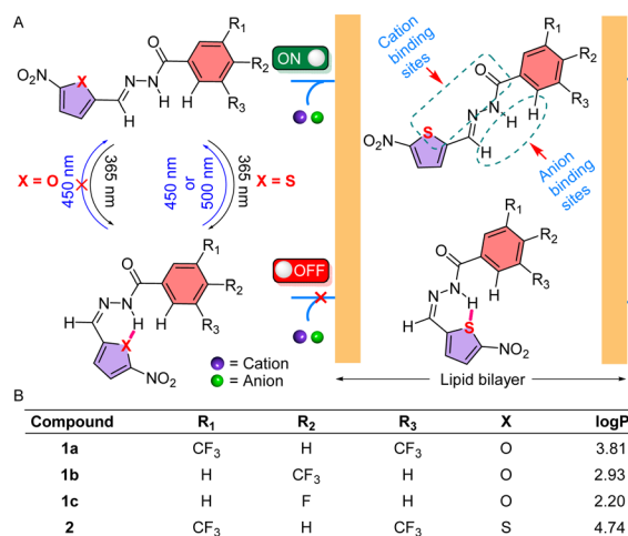
Fig. 1 Chemical structure of compounds 1a–1c and 2 with photoisomerization property and its effect on the ion transport process (A); structural description and log P values of designed molecules 1a–1c and 2 (B).
