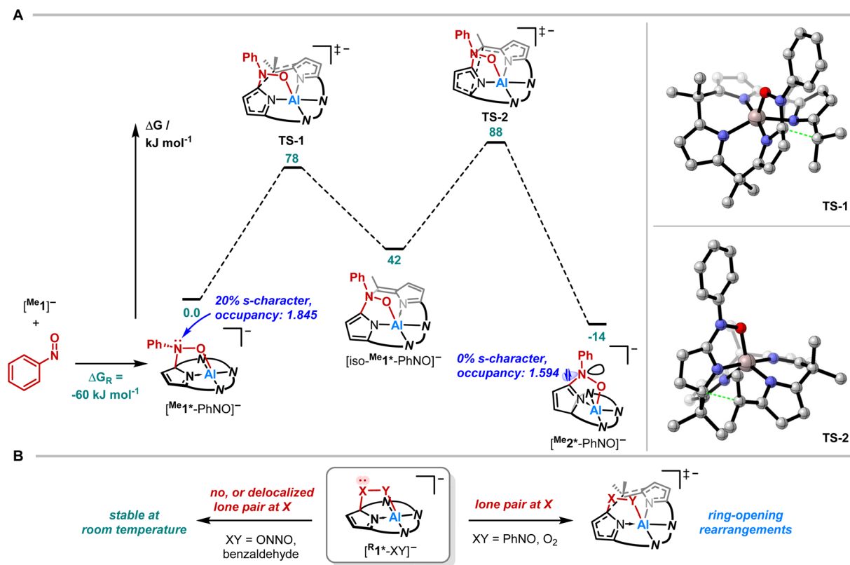
Fig. 5 (A) Computed reaction profile for the rearrangement of [\text{PPh}_4][\text{Me}1^* \text{-PhNO}] at the RI-DSD-PBEB95-D3(BJ)/def2-QZVPP, COSMO-RS( \text{CH}_2\text{Cl}_2 )/PBEh-3c level of theory and the respective transition structures. (B) Schematic representation on the influence of the presence of a lone-pair at the C-bound X on the stability of 1,2-adducts generalized as [\text{R}1^* \text{-XY}]^- .
