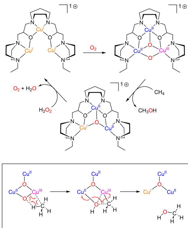
Scheme 13 Top: Catalytic cycle for the oxidation of \text{CH}_4 mediated by the [\text{Cu}^{\text{I}}\text{Cu}^{\text{I}}\text{Cu}^{\text{I}}(7\text{-N-Etpyz})]^{1+} complex and \text{O}_2 in the presence of hydrogen peroxide. Bottom: Proposed intermediates for methane oxidation. Adapted from ref. 227 and 229.
