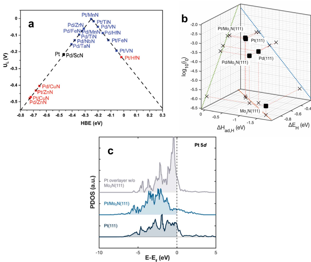
Fig. 7 (a) Volcano relationship for Pt-modified TMNs. (b) Correlation between the HER activity ( \log_{10}(j_0) ) and the binding strength of atomic hydrogen determined by TPD ( \Delta H_{\text{ad,H}} ) and DFT ( \Delta E_H ). (c) Projected density of states (PDOS) for Pt and Pt/TMN surfaces. (a) Reprinted from ref. 114 with permission from the Royal Society of Chemistry, Copyright 2022. (b and c) Reprinted from ref. 37 with permission from the American Chemical Society, Copyright 2023.
