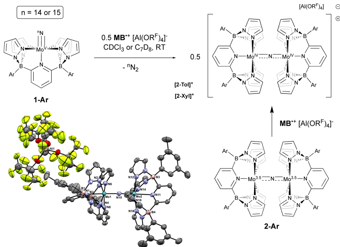
Fig. 3 Oxidation of neutral nitridos 1-Ar with 0.5 equivalents of [ MB ] + [Al(OR F ) 4 ] – . Lower left: molecular structure of [ 2-Xyl ] + [Al(OR F ) 4 ] – . Thermal ellipsoids are shown at the 50% probability level and all H atoms are omitted for clarity. Selected bond distances (Å): Mo(1)–N(10), 1.856(3); Mo(2)–N(10), 1.859(3); Mo(1)–N(1), 2.260(3); Mo(2)–N(11), 2.265(3). Selected bond angles (°): Mo(1)–N(10)–Mo(2), 176.52(19).
