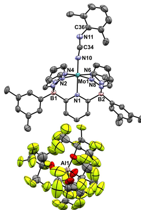
Fig. 6 Molecular structure of [4-Xyl] + . Thermal ellipsoids are shown at the 50% probability level and all H atoms are omitted for clarity. Selected bond distances ( \text{\AA} ): \text{Mo}(1)-\text{N}(1) , 2.167(3) ; \text{Mo}(1)-\text{N}(10) , 1.921(3) ; \text{N}(10)-\text{C}(34) , 1.210(5) ; \text{C}(34)-\text{N}(11) , 1.207(5) ; \text{N}(11)-\text{C}(36) , 1.391(6) selected bond angles ( ^\circ ): \text{N}(1)-\text{Mo}(1)-\text{N}(10) , 176.82(12) ; \text{Mo}(1)-\text{N}(10)-\text{C}(34) , 171.8(3) ; \text{N}(10)-\text{C}(34)-\text{N}(11) , 170.1(5) ; \text{C}(34)-\text{N}(11)-\text{C}(36) , 137.1(4) .
