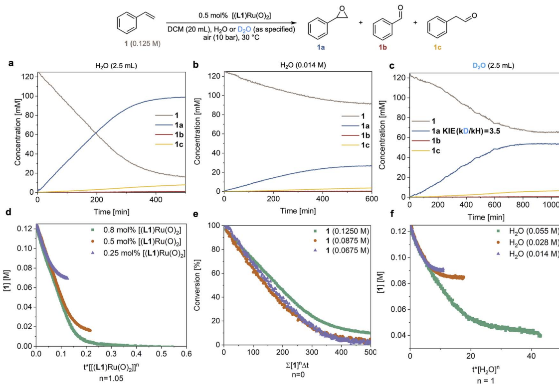
Fig. 3 Kinetic analysis from operando 1 H FlowNMR spectroscopy. (a) Reaction progress in DCM saturated with an excess of H 2 O. (b) Reaction progress in laboratory grade DCM (residual H 2 O content 14 mM). (c) Reaction progress in DCM saturated with an excess of D 2 O (99.9 atom% D). (d) Determination of the order in catalyst using VTNA. (e) Determination of the order in 1 using VTNA. (f) Determination of the order in H 2 O using VTNA.
