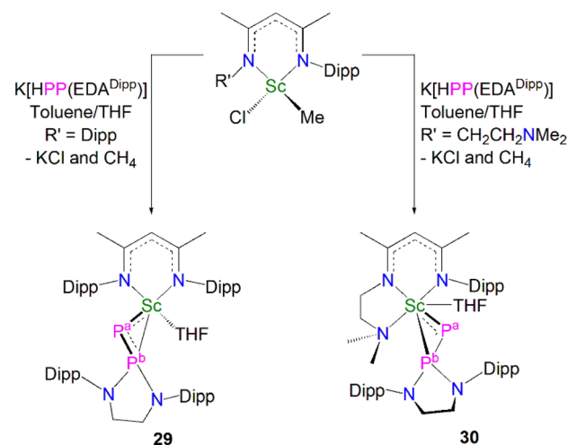
Scheme 11 Synthesis of the Sc-phosphinophosphinidene complexes 29 and 30 .
