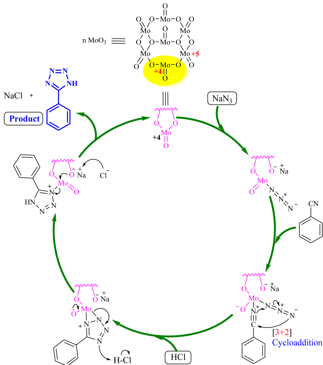
Fig. 5 Plausible mechanism for the synthesis of 5-substituted-1H-tetrazoles using MoO 3 .
