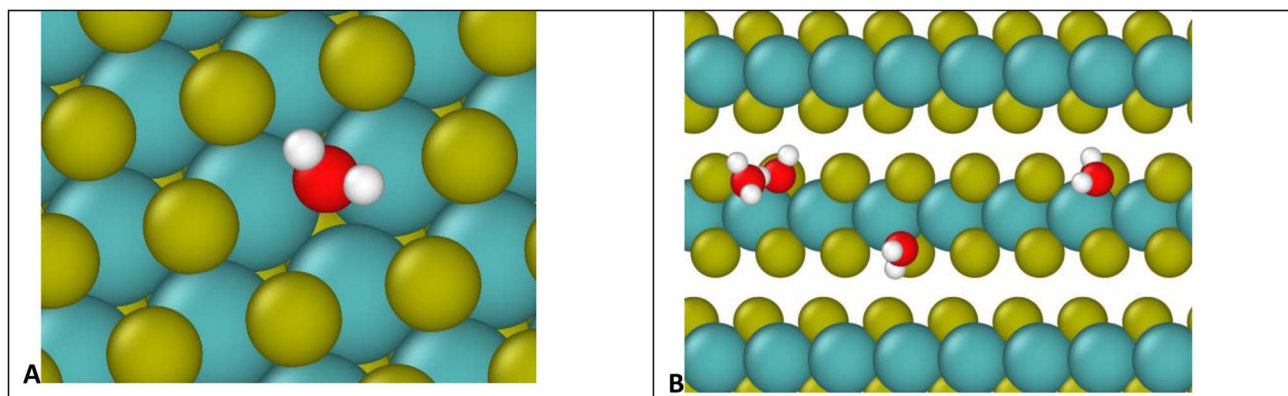
Fig. 9 Visualization of water molecules adsorbed to (A) defect on basal surface, (B) defects on an edge. Colors: yellow S, red O, white H, teal Mo. The relative sizes of the atoms are for clarity, and do not represent reality.
