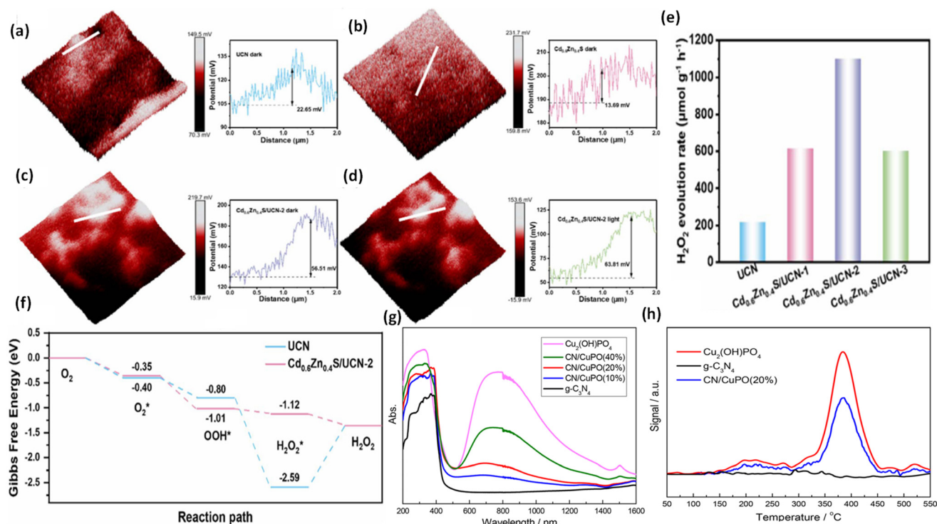
Fig. 25 3D surface charge potential distribution and corresponding line-scanning profiles of (a) UCN, (b) \text{Cd}_{0.6}\text{Zn}_{0.4}\text{S} , and (c) \text{Cd}_{0.6}\text{Zn}_{0.4}\text{S/UCN-2} composite in the dark, and (d) the \text{Cd}_{0.6}\text{Zn}_{0.4}\text{S/UCN-2} heterojunction photocatalyst under illumination. (e) Production rate comparison of UCN and \text{Cd}_{0.6}\text{Zn}_{0.4}\text{S/UCN} composites using visible light. (f) Free energy diagrams illustrating \text{O}_2 conversion to \text{H}_2\text{O}_2 by UCN and \text{Cd}_{0.6}\text{Zn}_{0.4}\text{S/UCN-2} systems. The figures are adapted with permission from ref. 11. Copyright 2023, RSC. (g) UV-vis spectra comparison of \text{g-C}_3\text{N}_4 , \text{Cu}_2(\text{OH})\text{PO}_4 , and \text{CN/CuPO}(20\%) samples. The figures are adapted with permission from ref. 198. Copyright 2018, ACS.
