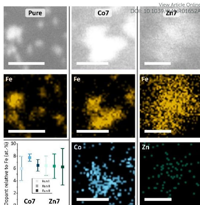
Figure 3 – (A) Representative EDX-STEM images of MFT (Pure) and doped (Co7, Zn7) samples. (B) Elemental maps for indicated elements Fe, Co, and Zn (scale bar: 50 nm). (C) The graph shows the dopant concentration relative to Fe of individual runs I-III.
