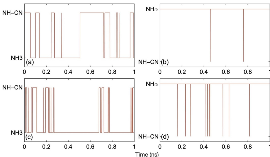
Fig. 4 Hydrogen hopping dynamics over 1 ns ML trajectories generated starting from (a) the most stable structure (NH-CN) at 300 K, (b) the least stable structure (N H \alpha ) at 300 K, (c) the most stable structure (NH-CN) at 400 K, and (d) the least stable structure (N H \alpha ) at 400 K. The y-axis presents the position of the hydrogen circled in the corresponding structures (a)–(d) of Fig. 1. The frequency of hydrogen hopping increases at higher temperatures. The N–H bond length ranges from 0.98– to 1.26 Å. Hydrogen hopping occurs when the N–H bond length exceeds 1.26 Å.
