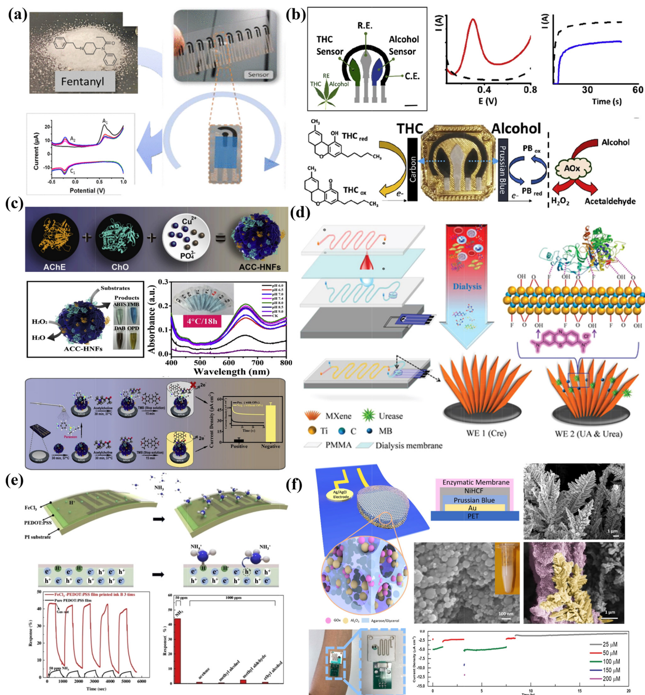
Fig. 6 Printable chemical sensors for analytes' rapid/on-site testing and their performance enhancements with nanomaterials. (a) Scalable fabrication of on-site illegal drug fentanyl sensors. Reproduced from ref. 156 with permission from [American Chemical Society], copyright [2019]. (b) Saliva sensing patch for on-site THC and alcohol dual analyte detection. Reproduced from ref. 40 with permission from [Elsevier], copyright [2020]. (c) Paper-based organophosphorus pesticide sensor with ultrasensitivity based on enzyme-inorganic hybrid nanoflowers and can generate electrochemical/colorimetric signals simultaneously. Reproduced from ref. 157 with permission from [Elsevier], copyright [2019]. (d) MXene-based screen-printed electrodes with a dialysis microfluidic chip for blood analytes monitoring without extra pretreatment. Reproduced from ref. 158 with permission from [John Wiley and Sons], copyright [2018]. (e) Inkjet printing of a PEDOT:PSS thin film with FeCl 3 additives for high performance ammonia gas sensing. Reproduced from ref. 159 with permission from [Elsevier], copyright [2019]. (f) Nanostructured glucose sensor with reliable long-term stability prepared on printed sweat sensing platforms. Reproduced from ref. 154 with permission from [John Wiley and Sons], copyright [2019].
