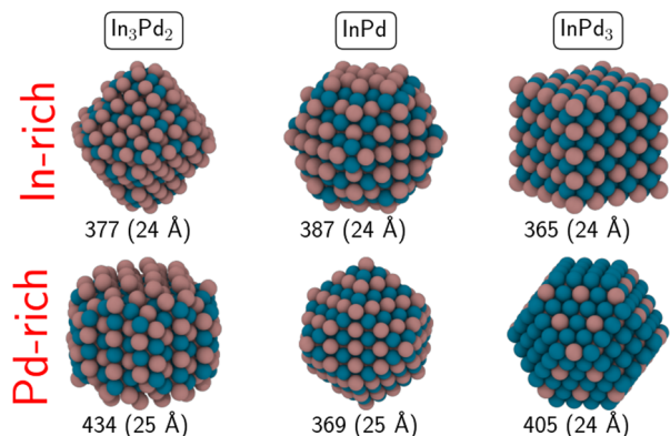
Fig. 3 Morphologies of \text{In}_3\text{Pd}_2 (left), \text{InPd} (middle) and \text{InPd}_3 (right) NPs based on the Wulff construction. The diameter of each NP is given, along with its number of atoms. The top row corresponds to the NP morphology at the In-rich side whereas the bottom row corresponds to the Pd-rich side. Colour code: Pd = blue and In = brown.
