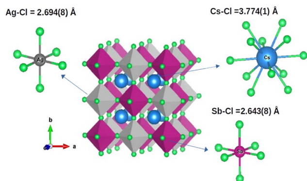
Fig. 4 Conventional unit cell of \text{Cs}_2\text{AgSbCl}_6 (space group Fm\bar{3}m ) showing the octahedra of the Sb (purple) and Ag (gray) sites; Cs (blue) shows the pseudo-octahedron. The interatomic distances of each \text{Cs}_2\text{AgSbCl}_6 element are extracted from Rietveld refinements.
