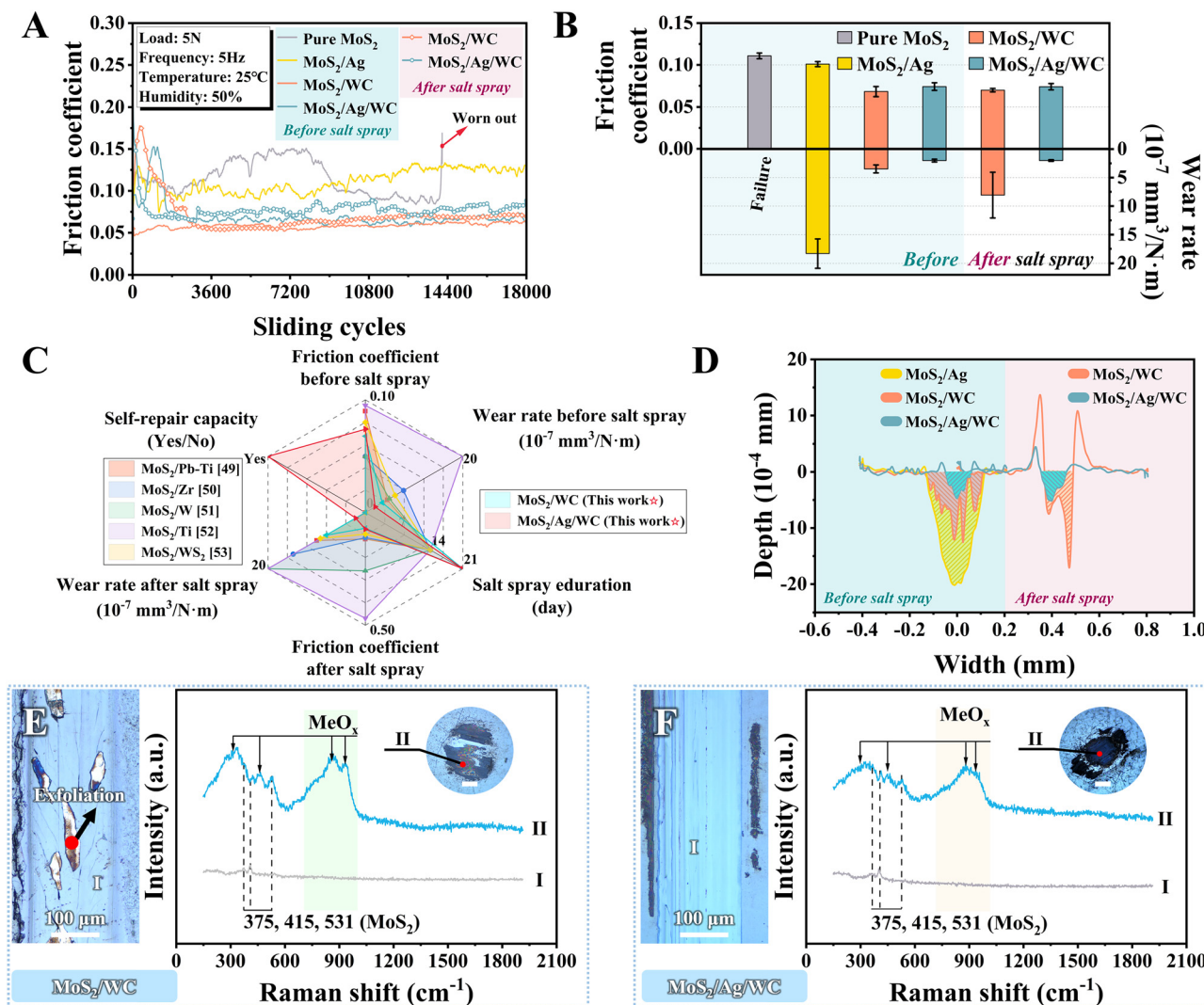
Fig. 8 Tribological properties of sandwich-like \text{MoS}_2/\text{Ag}/\text{WC} nanomultilayer film and reference films before and after salt spray tests. (A) and (B) Friction curves, average friction coefficients and wear rates before and after salt spray tests. (C) Comparison analysis of tribological performance of the sandwich-like \text{MoS}_2/\text{Ag}/\text{WC} nano-multilayer film versus previously reported \text{MoS}_2 -based films, both before and after salt spray testing. 49–53 (D) 2D profiles demonstrating the cross-sectional view of film wear tracks before and after salt spray tests, with slashes signifying the corresponding wear volume. (E) and (F) Optical images showing film wear tracks (I) and ball wear scars (II) of \text{MoS}_2/\text{WC} and \text{MoS}_2/\text{Ag}/\text{WC} nanomultilayer films after salt spray tests, with corresponding Raman spectra identified in marked positions. All the scale bars are of 100 \mu\text{m} .
