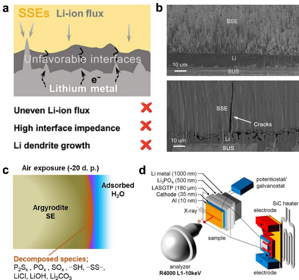
Figure 4. (a) Schematic of parasite reactions between SSEs and Li metal and the dendrite. 70 (b) Cross-section SEM image of interfacial evolution at SSE/Li before and after 20 cycles. 80 (c) Schematic of the decomposition of LGPS. 83 (d) Schematic of the ASSB and electrochemical setup for operando hard X-ray photoelectron spectroscopy (HAXPES). 91
