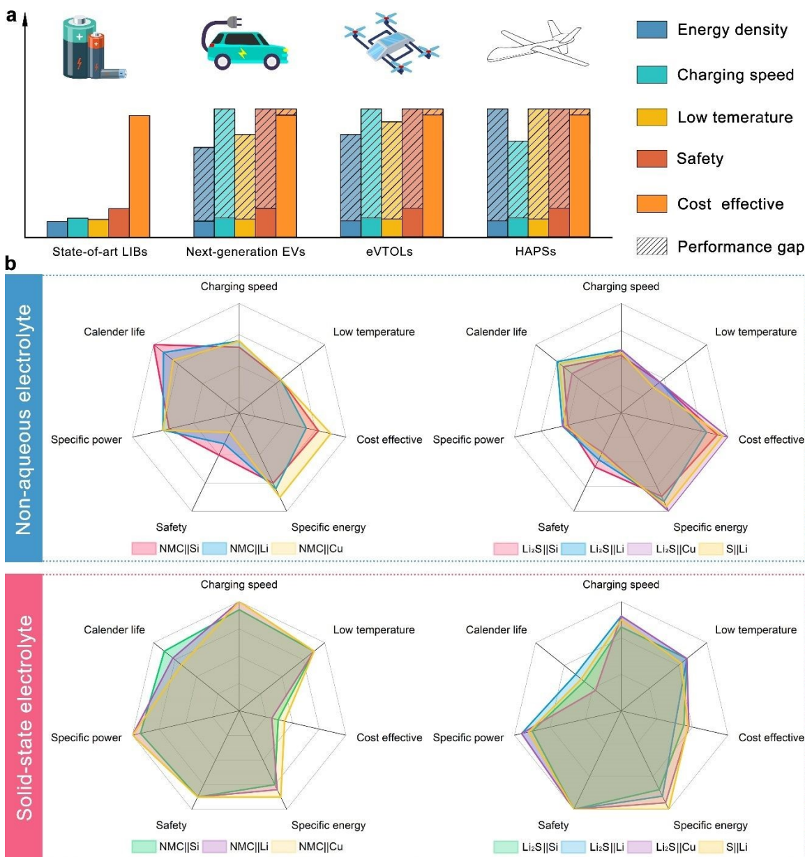
Figure 1. (a) Comparison of the requirements of next-generation EVs, eVTOLs, and HAPSSs with state-of-the-art LIBs in terms of energy density, charging speed, low-temperature performance, safety, and cost-effectiveness. (b) Radar plots of batteries with different configurations in both non-aqueous electrolytes and SSEs.
