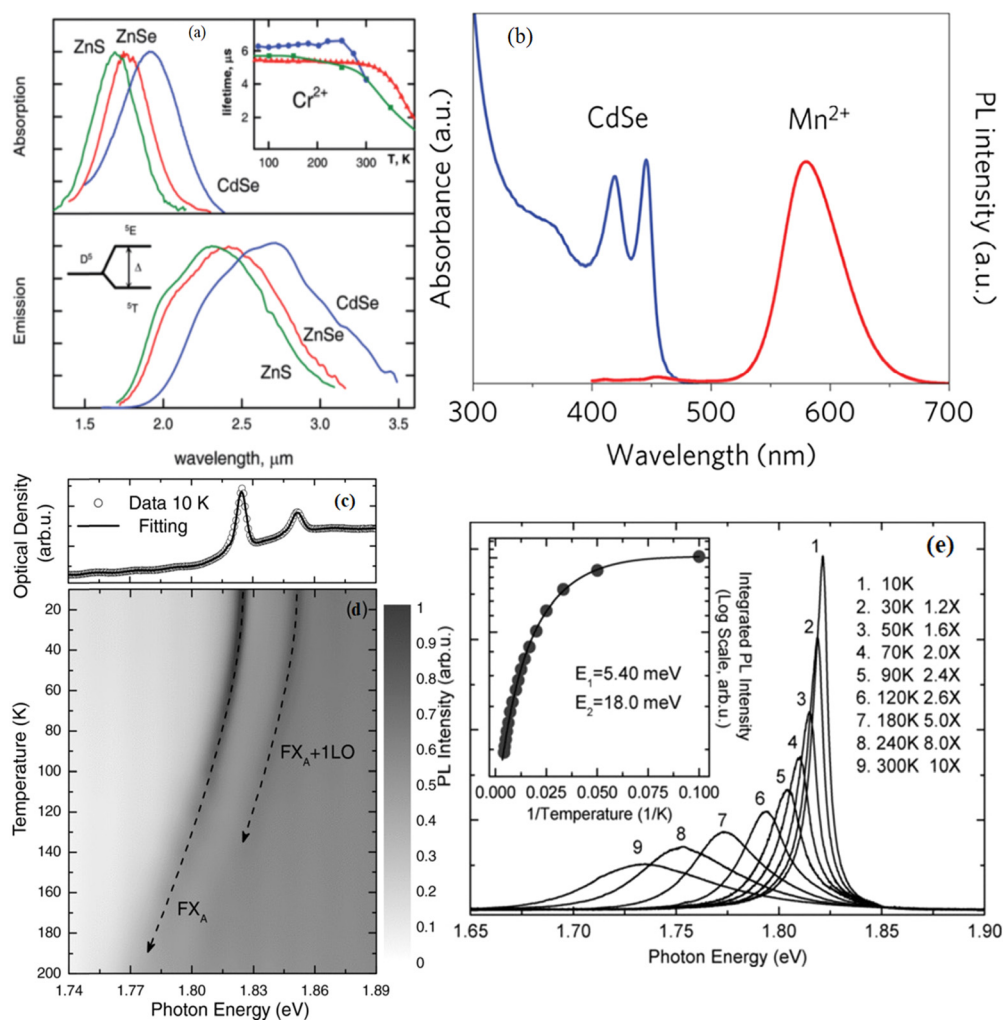
Fig. 4 (a) Normalized room temperature absorption and emission-gain spectra of Cr 2+ ions in ZnS, ZnSe, and CdSe crystals. Inset shows the temperature dependence of Cr 2+ ion lifetime in ZnS (circle), ZnSe (triangle), and CdSe (square) crystals; Copyright © 2010, Wiley InterScience. 133 (b) Absorption (blue line) and PL (red line) spectra of Mn-doped CdSe NPLs; Copyright © 2009, Springer Nature. 136 (c) Low temperature (10 K) free-exciton absorption of CdSe NWs. The solid curve is the multi-Gaussian fitting of the absorption spectrum. (d) Temperature-dependent mapping of the absorption spectrum. (e) Free-exciton emission of CdSe NWs at various temperatures. The inset plots the dependence of the integrated PL intensity on the reciprocal of temperature, and the solid curve is the Arrhenius fit with two activation energies, Copyright © 2011, Wiley. 145
