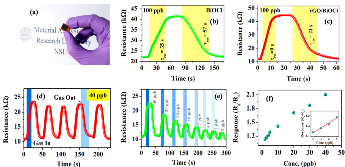
Fig. 7 (a) Thin film deposited over IDE, (b) and (c) response curve for BiOCl and rGO/BiOCl, (d) sensing repeatability curve for rGO/BiOCl, (e) variation in sensor response with different ppb levels and (f) the limit of detection for rGO/BiOCl.
