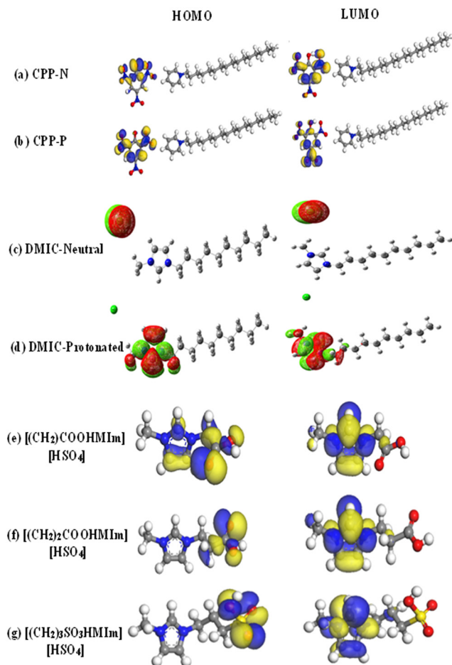
Fig. 14 Pictorial representation of the HOMO and LUMO orbitals of (a) CPP-N, (b) CPP-P, (c) DMIC-Neutral, (d) DMIC-Protonated, (e) [(\text{CH}_2)\text{COOHIm}] [\text{HSO}_4] , (f) [(\text{CH}_2)_2\text{COOHIm}] [\text{HSO}_4] and (g) [(\text{CH}_2)_3\text{SO}_3\text{HIm}] [\text{HSO}_4] (red colour: oxygen, grey colour: carbon, blue colour: nitrogen, white colour: hydrogen, yellow colour: sulphur). [Reprinted with permission from ref. 15, ©2023 Elsevier, ref. 39, ©2021 Elsevier, and ref. 115, ©2020 Elsevier.]
