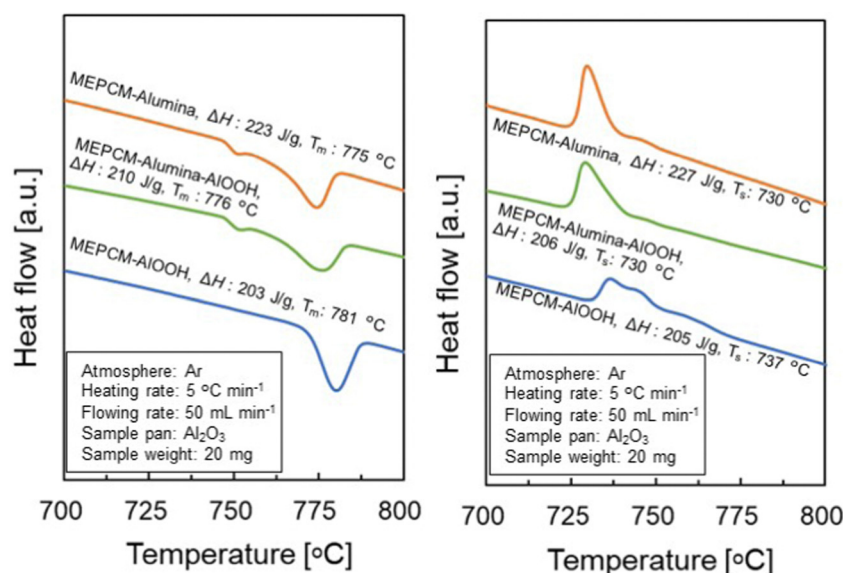
Fig. 5 DSC curve of various AIOOH addition MEPCMs after heat oxidation treatment. (T m : melting temperature of MEPCM, T s : solidification temperature of MEPCM, ΔH: latent heat storage capacity).
