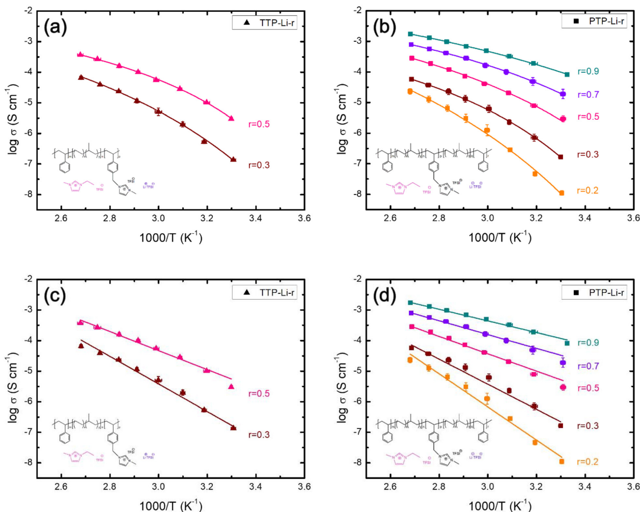
Fig. 5 Temperature-dependent ionic conductivity of the (a) TTP-Li-r, (b) PTP-Li-r with VFT regressions, (c) TTP-Li-r, and (d) PTP-Li-r with Arrhenius regressions at various r = [\text{IL}]/[\text{PIL block}] .
