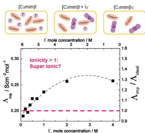
Fig. 5 Molar conductivity ( \Lambda_{imp} ) and ionicity ( \Lambda_{imp}/\Lambda_{ideal} ) of [C3mim] + I - with added I 2 as a function of I 3 - (I - ) concentration at iso-viscosity state of 0.2 Pa s. Reproduced from ref. 65 with permission from RSC, Copyright [2018].
