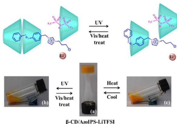
Fig. 47 (a) Mode of inclusion between β-CD and AzolPS-LiTFSI before and after UV irradiation. (b) Preparation of the supramolecular hydrogel: (a) β-CD/AzolPS-LiTFSI (3:1), and its disassembly induced by: (b) UV light, and (c) temperature. Reproduced from ref. 226 with permission from Wiley-VCH, Copyright [2018].
