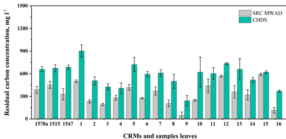
Fig. 5 Residual carbon contents (RCC, mg L -1 ) for CRMs (1570a, 1515, and 1547) and leaf samples obtained by the proposed closed vessel conductively heated digestion system (CHDS) and single reaction chamber microwave-assisted digestion (SRC MWAD).
