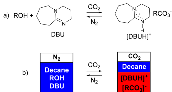
Fig. 3 A representation of a \text{CO}_2 switchable solvent (a), and the use of the technique for separations (b). Adapted from Jessop et al. 35 with permission from Springer Nature, 2024.
