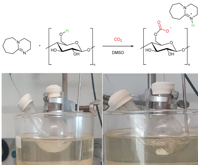
Scheme 1 (Top) The “derivative” switchable solvent method to solubilise cellulose. (Bottom) The dissolution of cellulose in a DMSO/DBU/ \text{CO}_2 mixture. Photo PMN, 2022.
