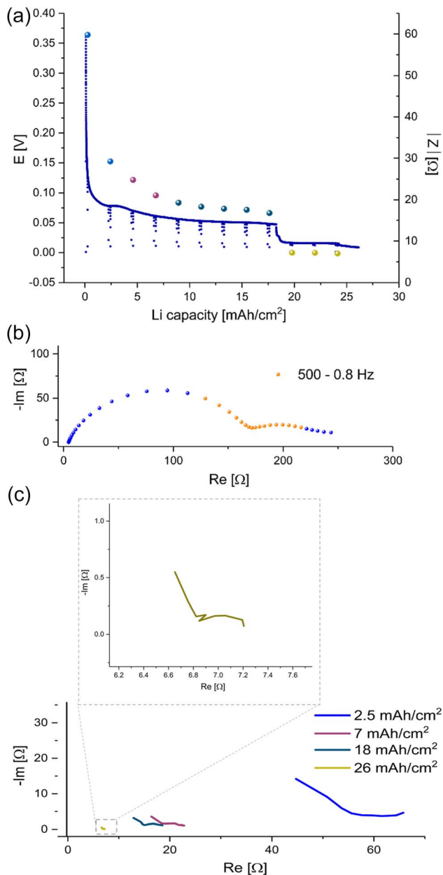
Fig. 4 (a) The voltage trace ( E-t ) of galvanostatic plating a total of 26 \text{mAh cm}^{-2} Li at 1 \text{mA cm}^{-2} in Li symmetric cell with LP30 electrolyte and GF separator at RT. EIS module values (spheres) were measured with GEIS at 9 Hz with 100 \mu\text{A} amplitude at 500–0.8 Hz. (b) A Nyquist plot of the PEIS spectrum of a symmetric lithium cell, LP30 electrolyte with GF separator measured after native SEI formation and before Li plating with 10 mV amplitude at RT. The frequency range used in the following GEIS measurements is indicated in orange. (c) Nyquist plots measured with GEIS, 100 \mu\text{A} amplitude at RT during Li plating in a symmetric cell, LP30 electrolyte RT with GF separator. Magnification of the plot measured after plating 26 \text{mAh cm}^{-2} Li.
