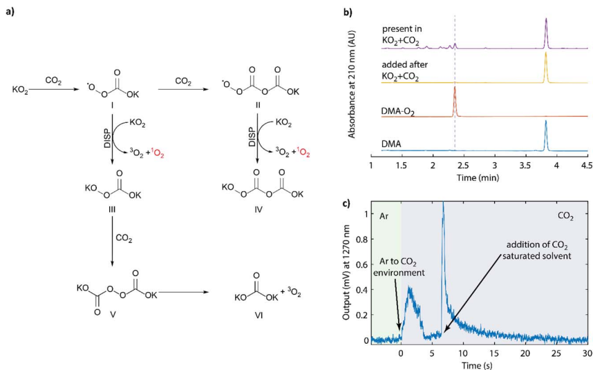
Fig. 4 (a) Reaction sequence upon reacting superoxide with \text{CO}_2 as initially described by Sawyer. 64 The final DISP step forming ^3\text{O}_2 was identified in this work. (b) HPLC elugram of DMA exposed to asymmetric \text{K}_2\text{C}_2\text{O}_6 (yellow trace) and DMA present during the reaction of \text{KO}_2 and \text{CO}_2 (purple trace). (c) NIR output signal around 1270 nm during the reaction of \text{KO}_2 with \text{CO}_2 . The \text{KO}_2 and 50 mM 18-crown-6 suspension in \text{CH}_3\text{CN} was initially kept under Ar, then the headspace was purged by \text{CO}_2 , and then \text{CO}_2 -saturated \text{CH}_3\text{CN} was added.
