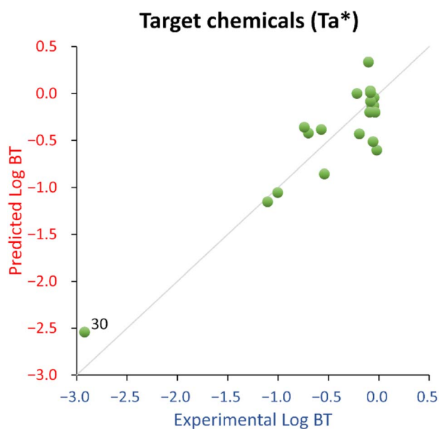
Fig. 2 Experimental vs. predicted log BT for the target chemicals (Ta*) QSPR. 30 = caffeine.
