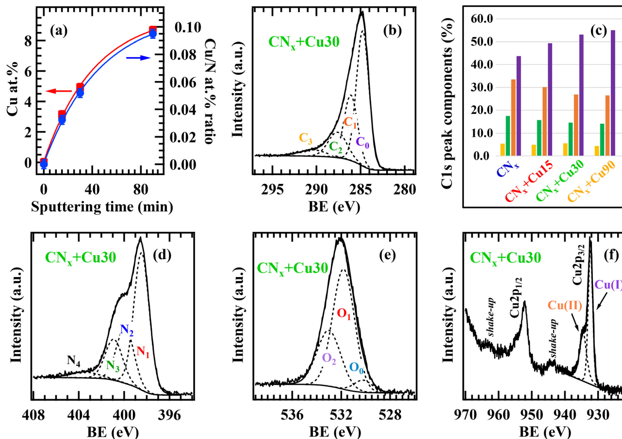
Fig. 3 (a) Cu at% and Cu/N atomic ratio vs. sputtering time (Cu at% was calculated excluding C and O). (b) Deconvoluted C 1s peak for the \text{CN}_x + Cu30 specimen. (c) Trend of the various C 1s peak components for the bare \text{CN}_x and Cu,O-functionalized samples, color codes are the same used for the C 1s bands in (b). (d) N 1s, (e) O 1s, and (f) Cu 2p photopeaks for the \text{CN}_x + Cu30 sample.
