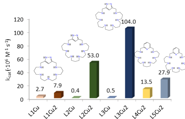
Fig. 12 Plot of the k_{\text{cat}} values for the mononuclear and binuclear Cu 2+ – L1 , Cu 2+ – L2 , Cu 2+ – L3 , Cu 2+ – L4 and Cu 2+ – L5 systems.
