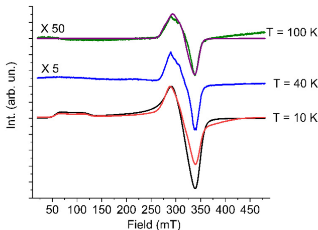
Fig. 2 Temperature dependence of the solid state EPR spectrum of 1 and best simulation for the T = 10 K spectrum (black line) and T = 100 K (purple line) obtained with models and parameters reported in the text. Spectra at 40 K and 100 K have been rescaled by factors reported on the left for a better appreciation.
