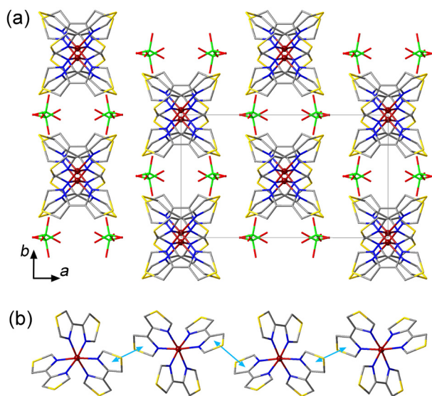
Fig. 1 (a) The crystal packing of 1 viewed down the c axis to reveal the columns of [\text{Fe}(4\text{bt})_3]^{2+} cations. The unit cell is indicated with solid gray lines. The H atoms are omitted for clarity. (b) A side view of a single column of cations, highlighting the \pi – \pi interactions with light-blue arrows. Color scheme: Fe = garnet, S = gold, Cl = green, O = red, N = blue, C = gray.
