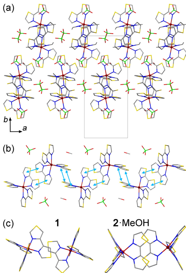
Fig. 2 (a) The crystal packing of 2-MeOH viewed down the c axis to reveal the columns of [\text{Fe}(2\text{bt})_3]^{2+} cations. The unit cell is shown with solid gray lines. The H atoms are omitted for clarity. (b) A side view of a single column of cations, highlighting the \pi - \pi interactions with light-blue double arrows. (c) The top view of \pi - \pi overlaps between the 4bt and 2bt ligands in 1 and 2-MeOH, respectively. Color scheme: Fe = garnet, S = gold, Cl = green, O = red, N = blue, C = gray.
