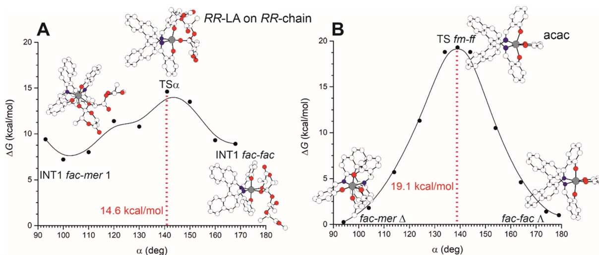
Fig. 4 Free energy profiles of the transformation from fac-mer \Delta to fac-fac \Delta for ( R )-1 as a function of the \text{O}_{\text{L}}\text{-Al}\text{-O}_{\text{L}} valence bond. The reorganization path moving from TS1 ( fm1 ) to TS2 ( ff ) as a function of \alpha for RR -LA polymerization is reported in A. The analogous path by using the bidentate acac − is reported in B. Aluminum, oxygen and nitrogen atoms in gray, red and blue. Hydrogen atoms have been omitted for clarity.
