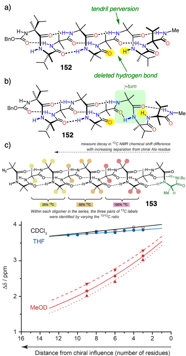
Fig. 74 (a) Tendrils perversions and (b) \gamma -turn in AIB foldamer 152 . (c) Chemical shift differences ( \Delta\delta ) measured in a series of three 'frame-shifted' oligomers, each containing three pairs of abundance-labelled (100%, 50% or 25%) ^{13}\text{C} labels. Screw-sense preference exhibited by Aib oligomer 153 decays as a terminal chiral influence becomes more distant. Reproduced from ref. 358 with permission from the Royal Society of Chemistry, copyright 2016.
