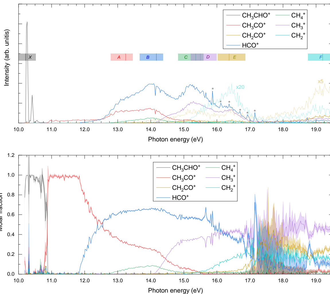
Fig. 4 (a) Threshold photoelectron spectra (TPES) for the parent ion and for the different fragment ions. The spectra for \text{CH}_2\text{CO}^+ and \text{CH}_2^+ were multiplied by factors of 5 and 20, respectively, and depicted with light lines. Colored vertical bars indicate vertical excitation energies reported by Cvitas et al. 6 The colored horizontal bands illustrate the approximate position of each band based on Refs. 6 and 7 . The peak observed at 14.2 eV is assigned to resonant excitation of Ar 5s present in the gas filter. * indicates autoionizing resonances from residual \text{N}_2 . (b) Molar fraction as a function of the photon energy. The error bars in panel (b) are estimated by propagating the experimental error from the TPES in panel (a), which in turn are derived assuming a Poisson distribution on the individual pixel counts of the photoelectron images. The large error bars in the 17–19 eV photon energy range are due to the particularly large cross-section of autoionizing states of residual \text{N}_2 . Note that, since only events related to the production of threshold electrons are considered, photon energy equals internal energy of the molecule.
