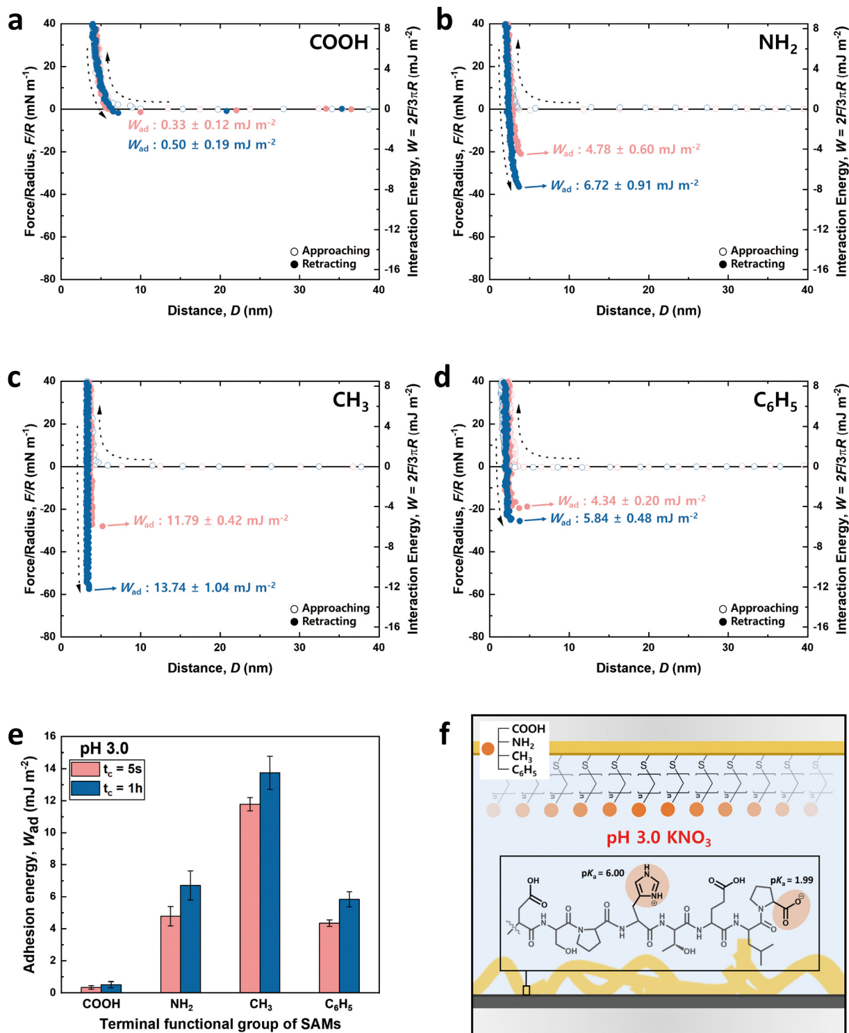
Fig. 3 Approaching and retracting force–distance profiles between the 8-mer peptide and functionalized SAM surfaces at pH 3.0. Four different functionalized SAMs are utilized: (a) –COOH, (b) – \text{NH}_2 , (c) – \text{CH}_3 , and (d) – \text{C}_6\text{H}_5 . (e) Bar graphs show the adhesion energy of the 8-mer peptide against four different SAMs as a function of contact time; average \pm standard error bars ( n > 3 ). (f) A peptide schematic showing the charged state of amino acids at pH 3.0.
