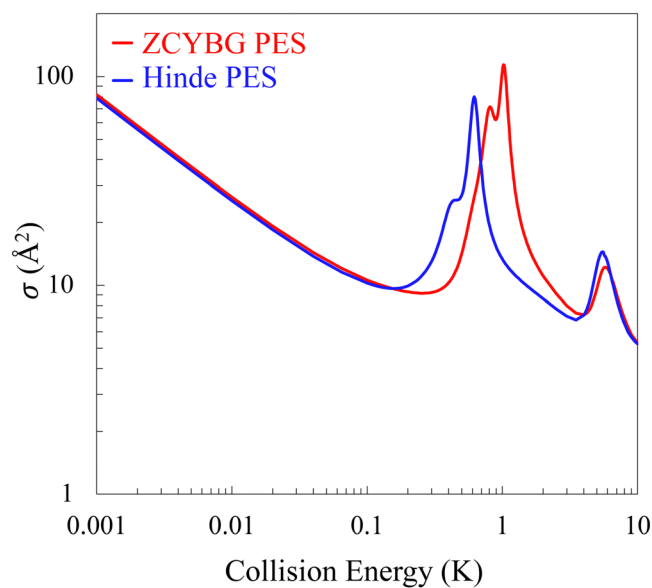
Fig. 7 Collision energy dependence of the inelastic cross section for \Delta j_{\text{HD}} = -1 transition in HD( v_{\text{HD}} = 1 ). The blue and red curves represent the results obtained on the Hinde and ZCYBG PESs, respectively.
