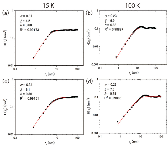
Fig. 5 Plots of HHCF analysis with fitting results using topographic data at (a) and (c) 15 K and (b) and (d) 100 K. (a) and (b) The results for x -direction analysis and (c) and (d) those for y -direction analysis.
