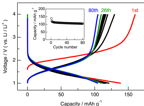
Fig. 3 Charge/discharge curves for \text{Li}_2\text{NbHO}_2 electrode between 1.0 and 4.0 V (vs. \text{Li}^+/\text{Li}^+ ) at a rate of C/10 ( = 38.3 \text{ mA g}^{-1} ) at 25^\circ\text{C} . Inset: Discharge capacity retention upon cycling up to 80 cycles. Li metal foil was used as the counter electrode, and 1 M \text{LiPF}_6 dissolved in a 1 : 1 v/v mixture of ethylene carbonate/diethyl carbonate (EC/DEC; Kishida Chemical) was employed as the electrolyte. Working electrode was formulated with 83 wt% active materials, 10 wt% acetylene black, and 7 wt% polytetrafluoroethylene (PTFE).
