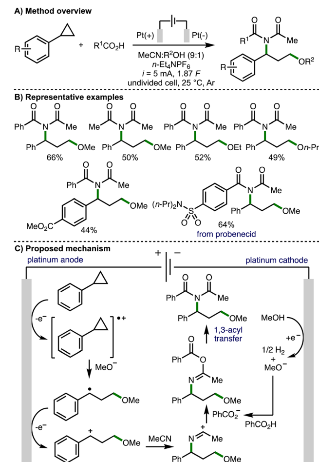
Scheme 10 1,3-Alkoxyimide of arylcyclopropanes (Luo and Xiao).
