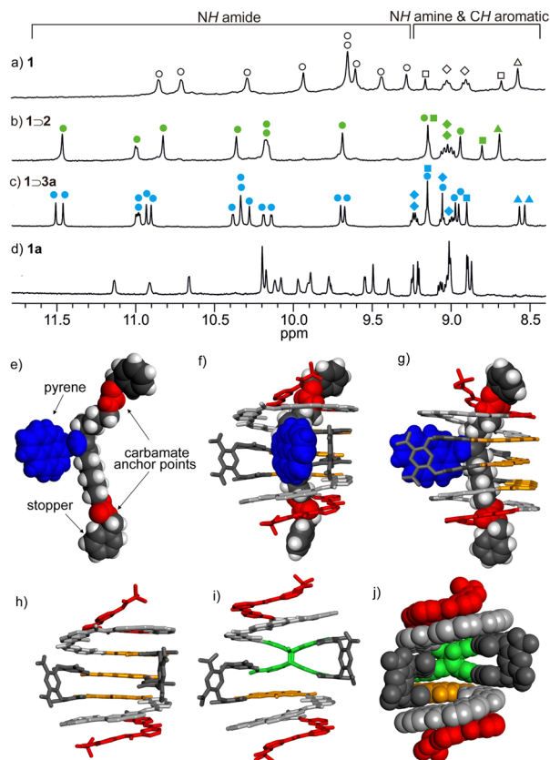
Fig. 3 Part of the 1 H NMR spectra (CD 2 Cl 2 , 400 MHz) of: (a) 0.5 mM 1 in absence of guest; (b) 0.5 mM 1 in the presence of 2 (5 equiv.); (c) 0.5 mM 1 in the presence of 3a (5 equiv.); (d) 1a . NH amide protons, NH amine protons, CH aromatic protons from A H unit (H9 and H10) and H ext are marked as circles (O), diamonds (◊), squares (◻) and triangles (Δ), respectively. Signals of the free symmetrical host, symmetrical foldaxane 1 ⊃ 2 and unsymmetrical foldaxane 1 ⊃ 3a are marked and filled with empty, green, and blue circles, respectively. Structures in the solid state analysed by X-ray crystallography of: (e) T-shape guest in the crystal packing; and (f) front view and (g) side view of foldaxane 1 ⊃ 3a . The guest is shown as a CPK representation and the host is shown as a stick representation. (h) Host 1 as it exists in the structure of 1 ⊃ 3a . Front view of the energy-minimised molecular models (using Merck molecular force field static, MMFFs) of 1a in stick representation (i) and CPK representation (j). The carbamate and pyrene in the T-shape guest are marked in red and blue, respectively. The monomers in the host are colour coded as in Fig. 2. Side chains (O t Bu groups) of host and included solvent molecules have been removed for clarity.
