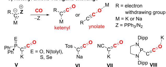
Fig. 1 (A) In situ formation of a lithium ynoate by carbonylation of metalated a diazomethane. (B) Formation of ketenyl anion from the reaction of a dilithiomethandiide with CO and N 2 O or (C) via PPh 3 /CO exchange and examples of isolated ketenyl anions.
