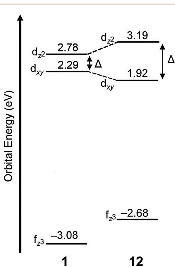
Fig. 8 Calculated d-orbital splitting of \text{Eu}^{\text{II}}\mathbf{1} and \text{Eu}^{\text{II}}\mathbf{12} . Adapted from Corbin et al., 81 copyright 2018, with permission from Elsevier.
