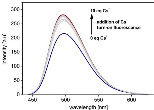
Fig. 3 Fluorescence Cs + titration of representative bowl-shaped and N-doped PAH receptor 1 ( \lambda_{\text{ex}} = 320 nm).
