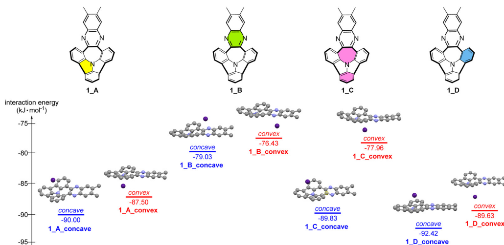
Fig. 4 Graphical presentation of the interaction energies for the systems comprising Cs + and 1 , together with the computed complexes' arrangements (hydrogen atoms are omitted for the clarity of the images). Considered parts of receptor 1 included in the Cs + binding process are marked with colours.
