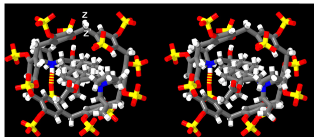
Fig. 3 Cross-eyed stereoview of an MMFF minimized geometry of the P6MQ ·roc complex. Color code: C, grey; H, white; N, blue; O, red; H-bonds, red-yellow stripped.
