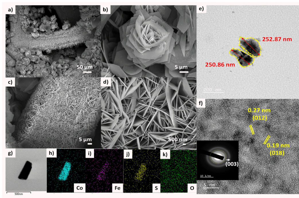
Fig. 2 FESEM images of (a) and (b) S-CoFeLDH/NF and (c) and (d) CoFeLDH/NF at different resolutions. (e) TEM image, (f) HR-TEM image with the inset showing the SAED pattern of S-CoFeLDH/NF and (g)–(k) elemental maps of Co, Fe, S and O of S-CoFeLDH/NF.
