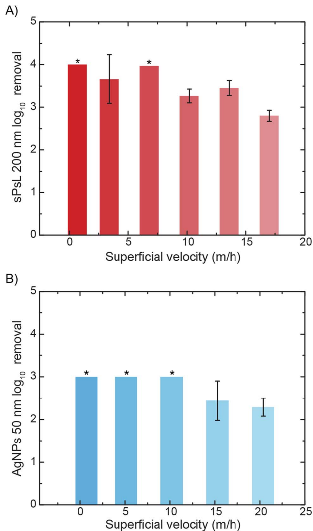
Fig. 3 MO-functionalized cotton filters show high efficiencies of nanoparticle removal at superficial velocities typical in drinking water treatment. (A) Experimental log 10 removal of sPSL particles using MO-functionalized cotton filters at various flowrates in the range of 2 mL min -1 to 50 mL min -1 showed that MO-cotton filters achieve 2.80 \pm 0.13 log 10 removal of sPSL particles at a flow rate of up to 50 mL min -1 which corresponds to a superficial velocity of 16.98 m h -1 (B) Experimental log 10 removal of AgNPs using MO-functionalized cotton filters at various flowrates in the range of 2 mL min -1 to 60 mL min -1 showed that MO-cotton filters achieve 2.29 \pm 0.21 log 10 removal of AgNPs at a flow rate of up to 60 mL min -1 which corresponds to a superficial velocity of 20.37 m h -1 . When compared to the typical operating conditions of two widely used conventional filters, rapid sand filtration (5–15 m h -1 ) and slow sand filtration (0.1–0.4 m h -1 ), MO-functionalized cotton filters show the potential to be applicable in conventional water treatment. *Indicates that the effluent concentration was below the limit of detection which indicates that the actual removal, in this case, could be higher than the reported values. Error bars represent the standard deviation calculated from three independent measurements.
