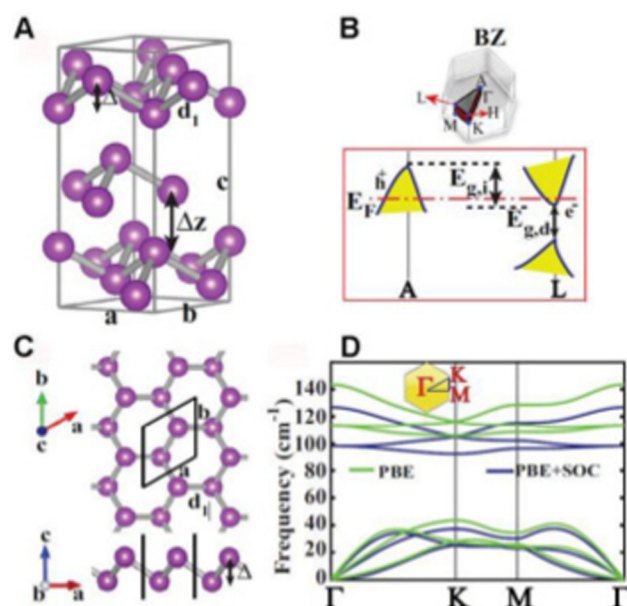
Fig. 4 (A) Hexagonal unit cell of bulk Bi structure, (B) related structure of Bi crystal, (C) single-layer of buckled honeycomb structure of Bi, b-Bi and a-Bi and (D) phonon dispersion curves calculated with and without spin-orbit coupling. Reprinted with permission from ACS. 12
